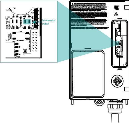
Figure 16. ModBus Termination Switch*
