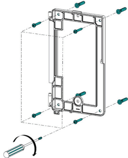
Figure 5. Alternate Bracket Mounting
