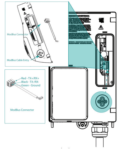
Figure 14. Serial RS485 ModBus Connection*
