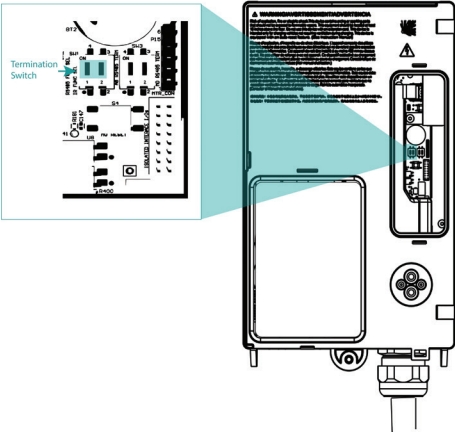
Figure 15. Commercial ModBus Termination Switch*
