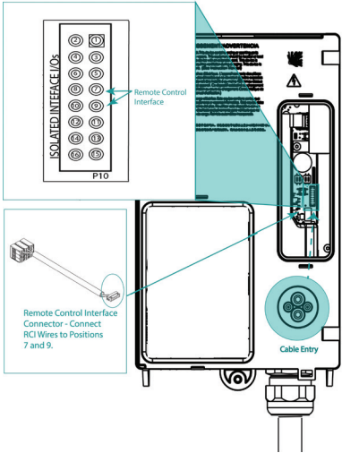
Figure 17. External Remote Control Interface**
