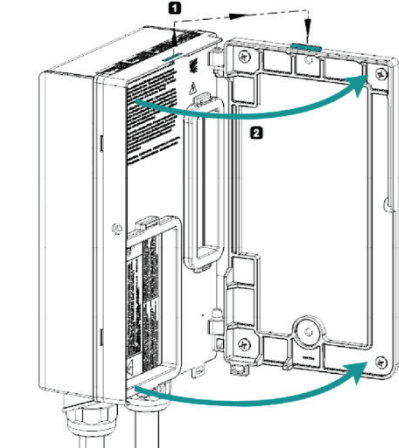
Figure 8. Close Charger
