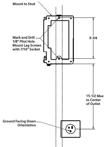
Figure 3. Bracket Position
