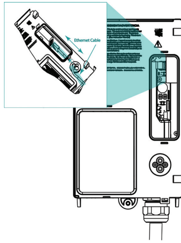
Figure 13. CAT6 Ethernet Port Connection**
