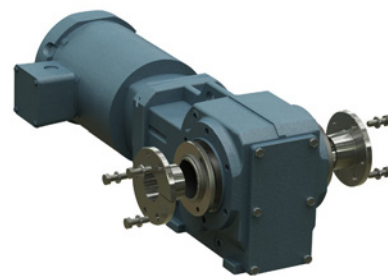
Twin tapered bushings
