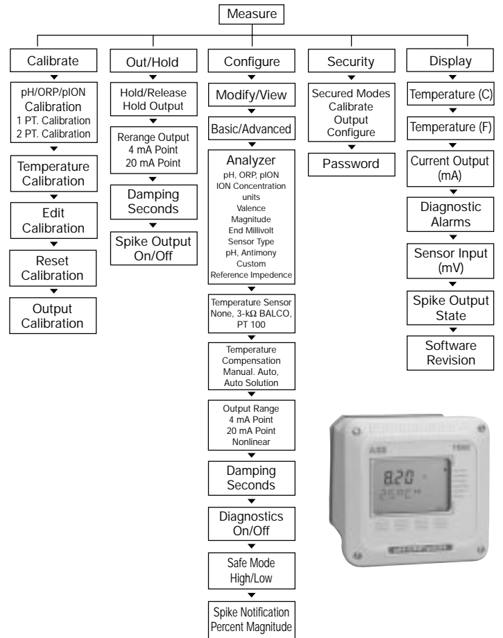
Flow Tree for the TB82pH/ORP/pION Advantage Transmitter
