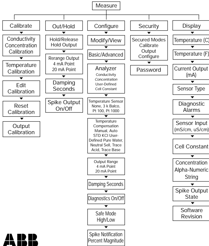
Flow Tree for the TB82TE Two-Electrode Advantage Conductivity Transmitter
