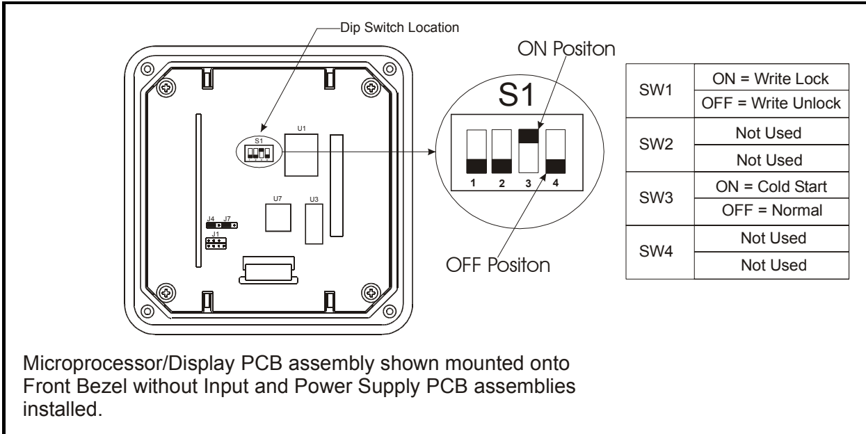
Figure 35 – Hardware Dip Switch Location and Function
