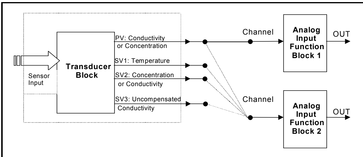
Figure 34 - Possible Connections Between the TB and AI's
