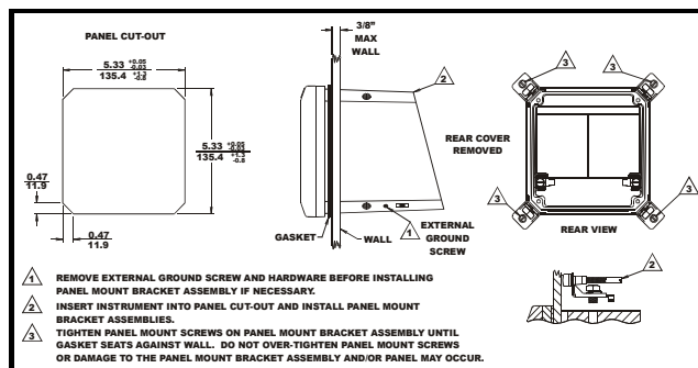
Figure 8 – Panel Mounting Detail
