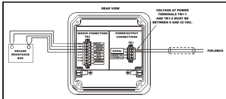
Figure 36 – Sensor Simulation Setup
