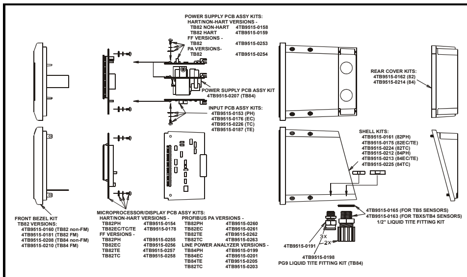
Figure 37 - TB82EC PA Transmitter Exploded View
