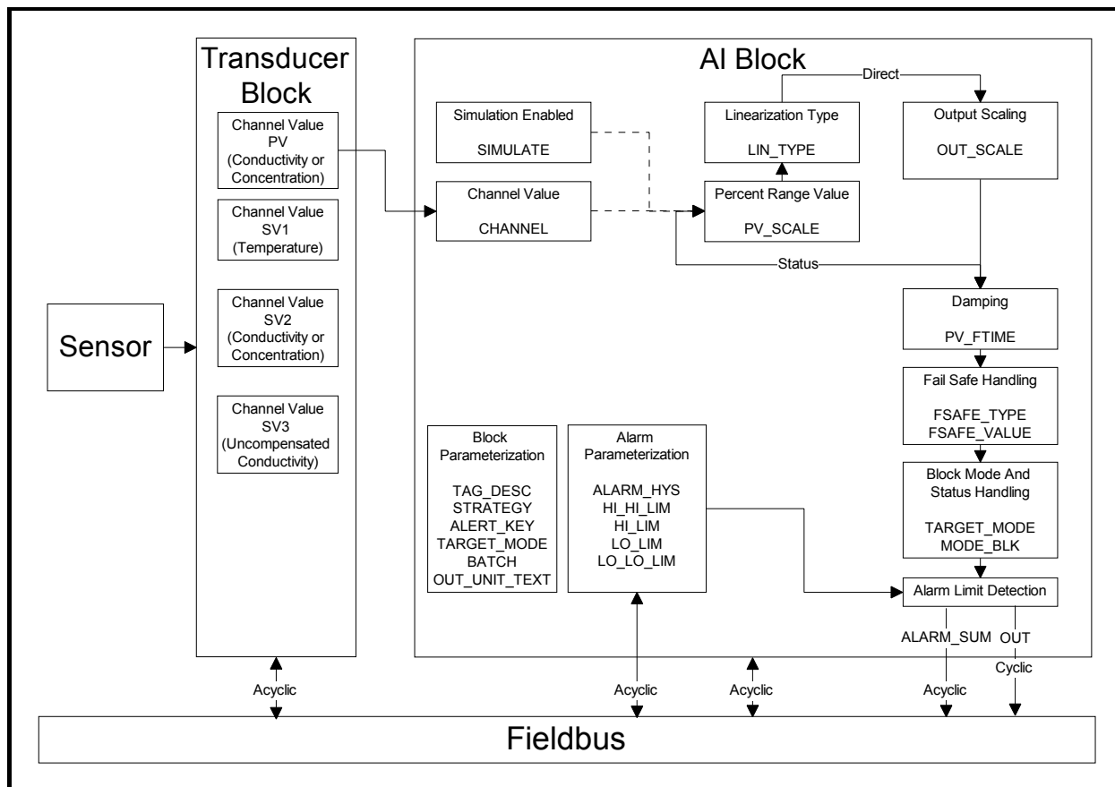
Figure 32 – Analog Input One Function Block Design Diagram
