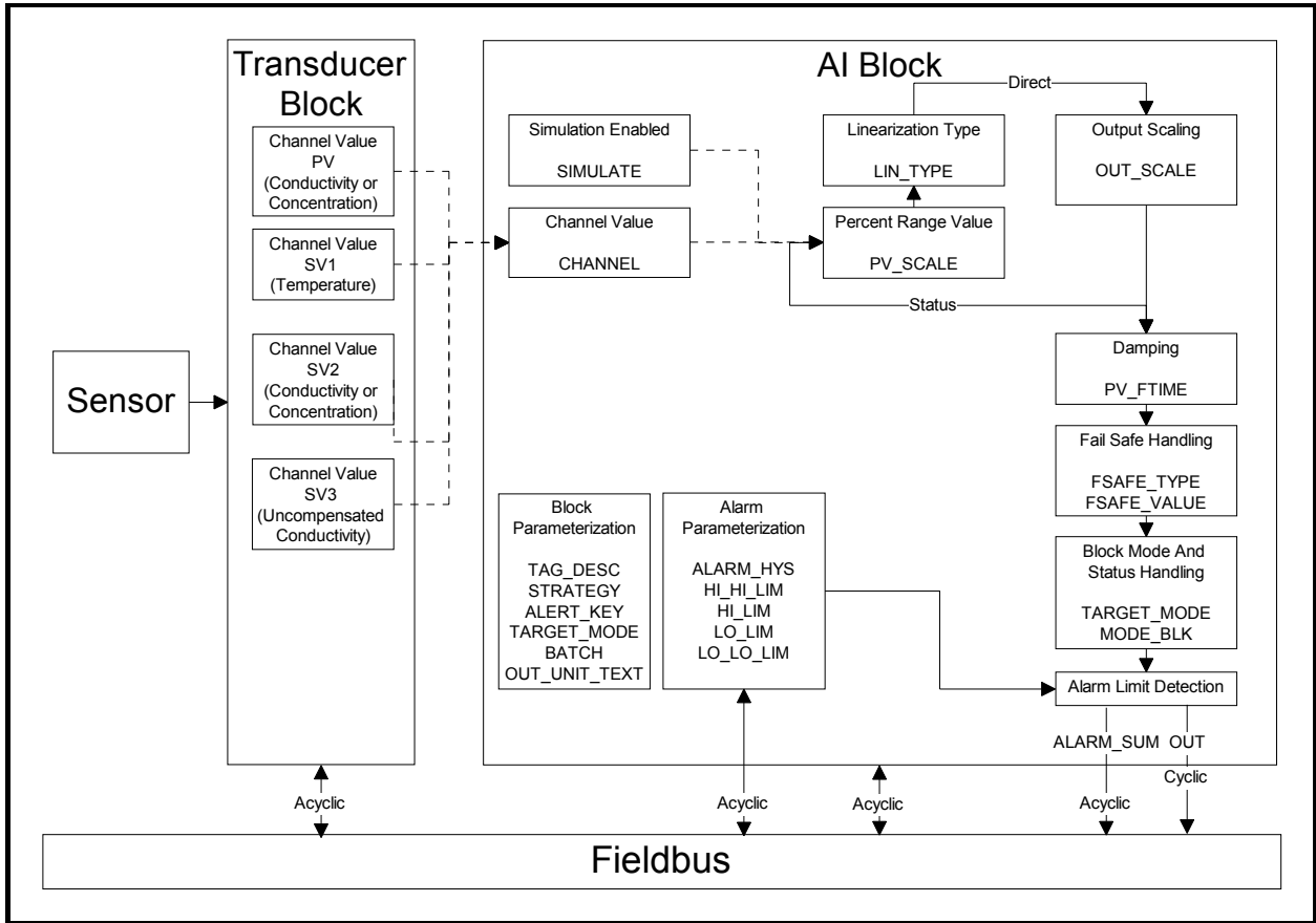
Figure 33 – Analog Input Two Function Block Design Diagram
