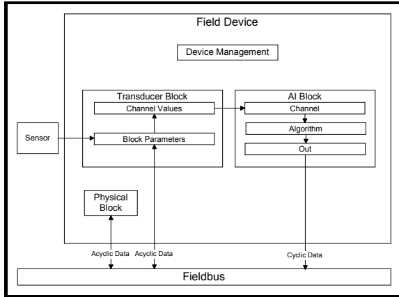
Figure 30 – Function Block Model Diagram
