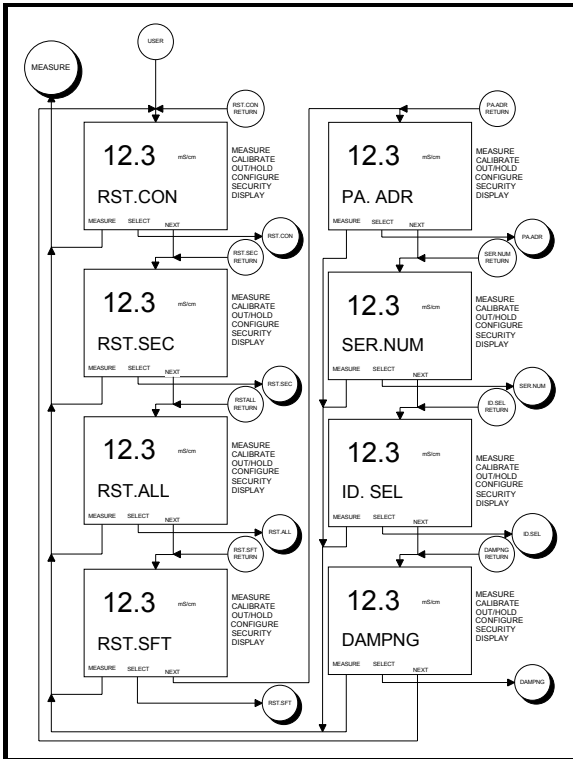
Figure 29 – Screen Flow Diagram for User States of Operation
